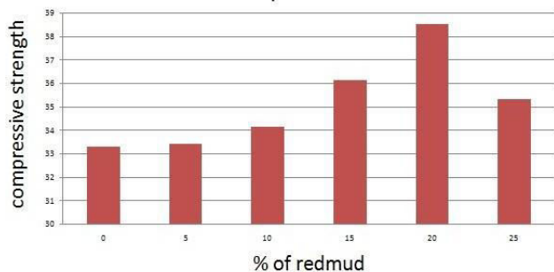
Figure1: COMPRESSIVE STRENGTH
